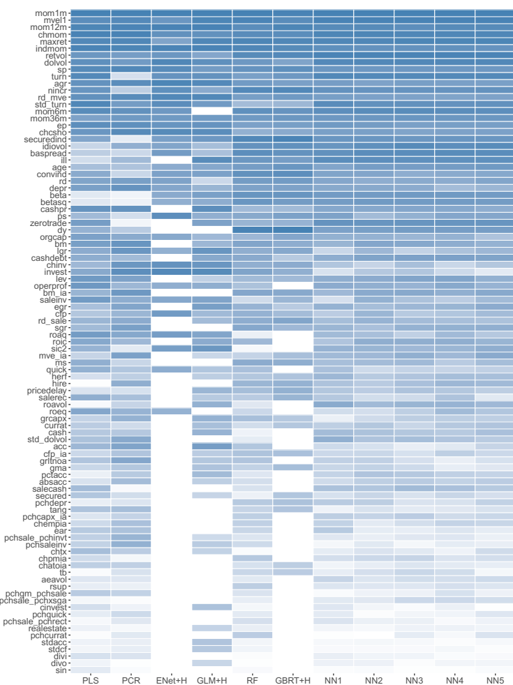
Figure 5 Characteristic importance
